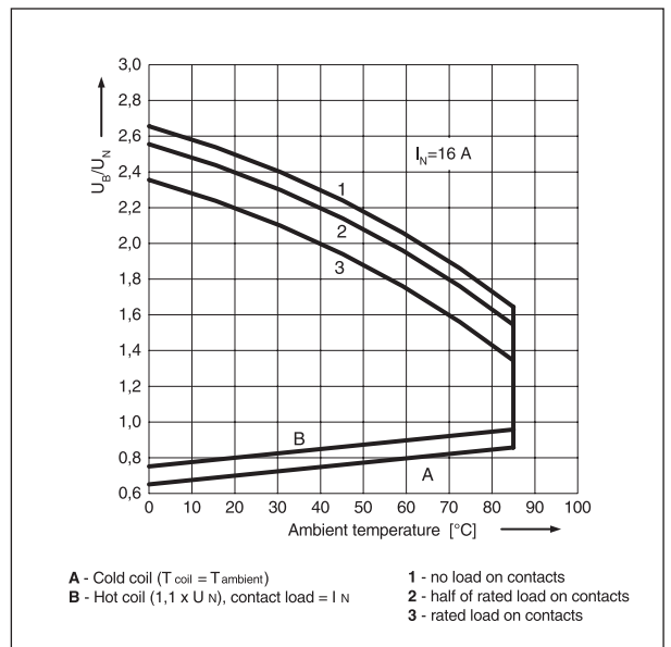
Coil operating range Fig. 4
